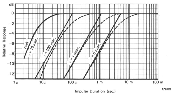
Fig. 4.10. Standard and optional "Peak Hold" responses of 2209
