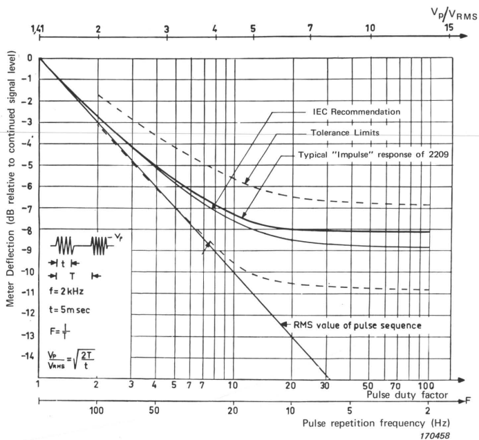
Fig. 4.9. Response of the 2209 to repeated impulses
