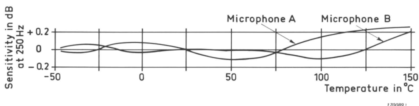
Fig.5.13. Sensitivity change of 4145 with temperature
