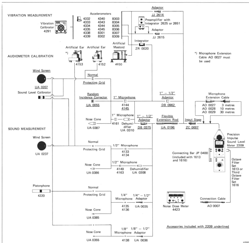
Fig.6.1a. Accessories for sound and vibration measurements
