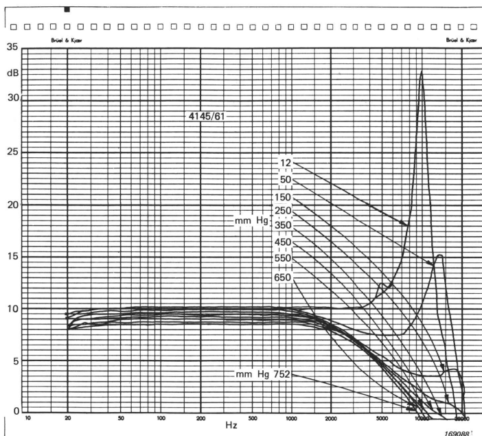
Fig. 5.21. Microphone frequency response with varying air pressure
