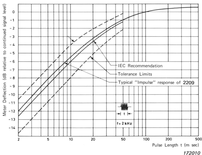
Fig. 4.8. Response of the 2209 to single impulses
