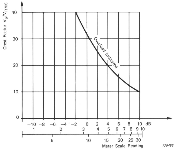
Fig. 5.11. Maximum Crest Factor at given meter deflection
