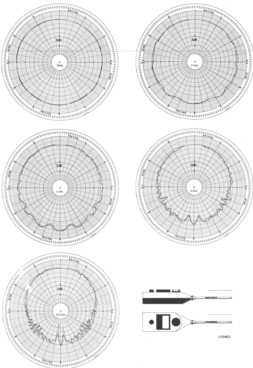
Fig.5. 4. Directional characteristics of 2209 with UA 0196 and 4133
