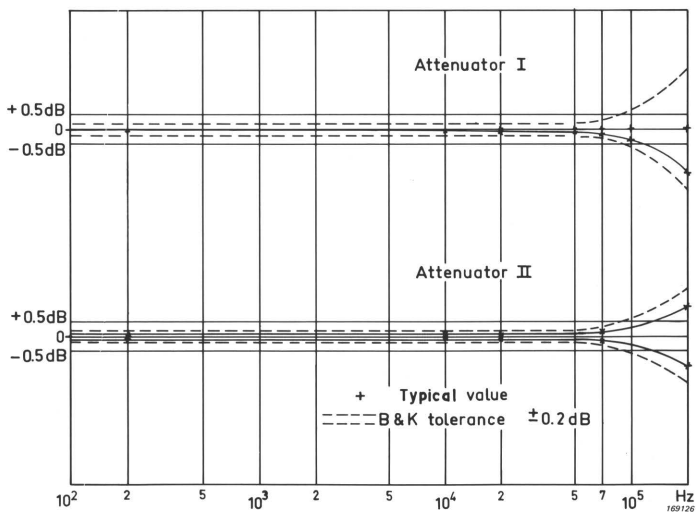
Fig.5.23. Attenuator frequency characteristics
