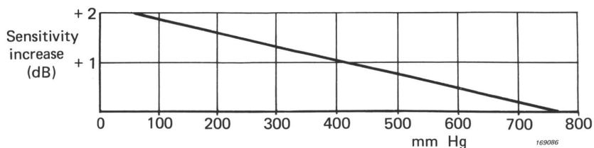
Fig.5.20. Change in Microphone sensitivity with ambient air pressure
