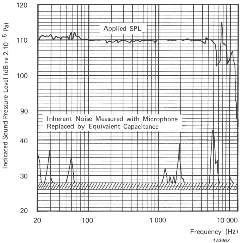
Fig.5.18. Influence of a sound field
