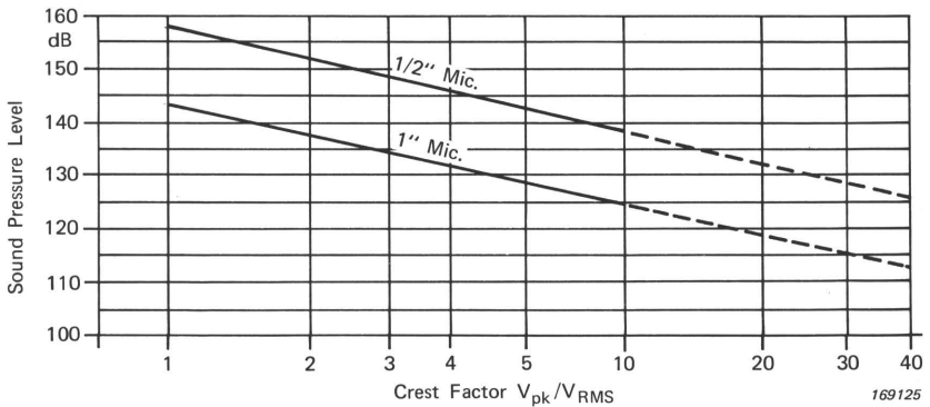
Fig. 5.12. Maximum SPLs that can be accurately measured with one-inch and half-inch microphones with respect to signal crest factor
