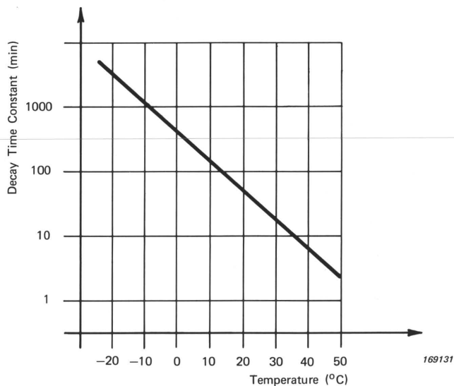
Fig.4. 12. Decay time vs. temperature for "Hold" circuit
